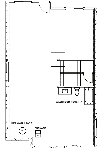
UNDEVELOPMENT BASEMENT
